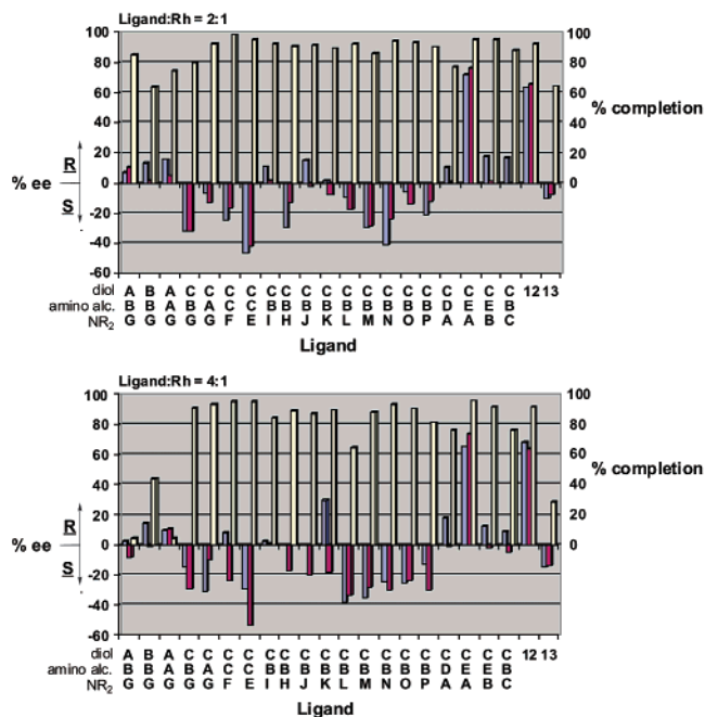
FIGURE 1. Results of hydrosilylation of 1-acetonaphthone with a selection of chiral ligands. Key: yellow, percent completion as measured by HPLC; blue, % ee as measured by the kinetic resolution/mass spectrometry (MSEED) method; red, % ee as measured by chiral HPLC (Chiralcel OD).
